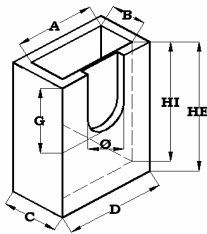
IMBORNAL
